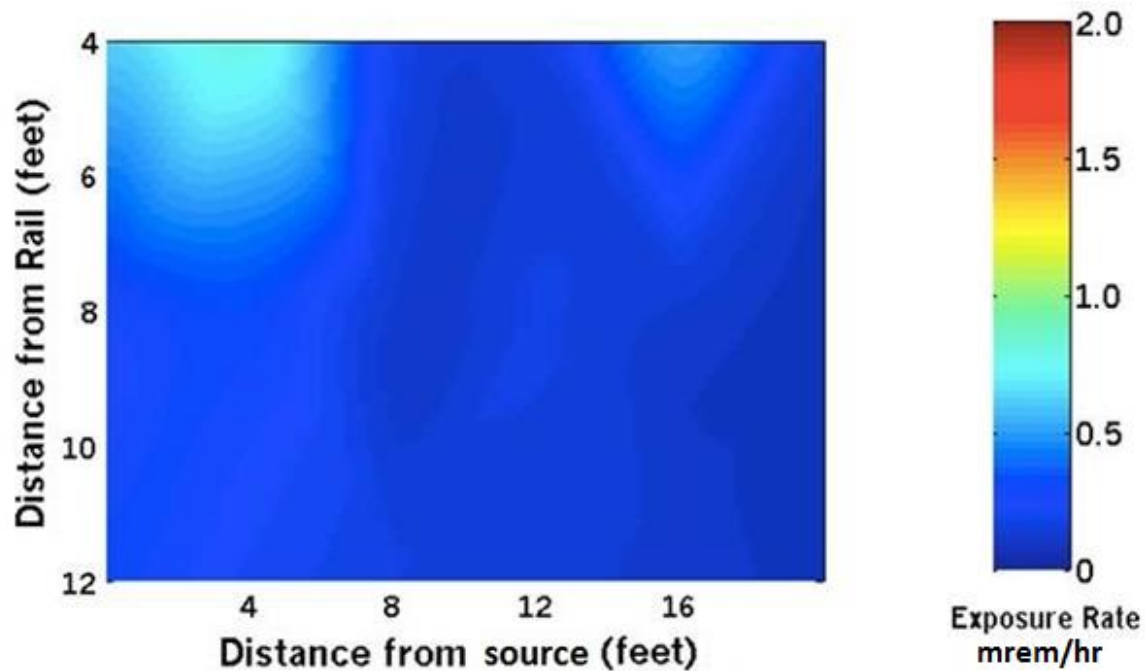
Figure 12: Plot of exposure rates 6 feet above the surface of the tie.
