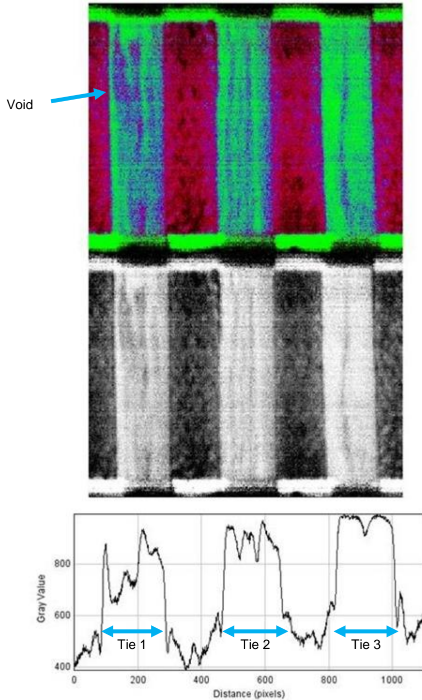
Figure 7: Various images of 3 used wood ties. Top: Colored image. Middle: Grayscale Image. Bottom: Average Density Profile in the longitudinal direction.
