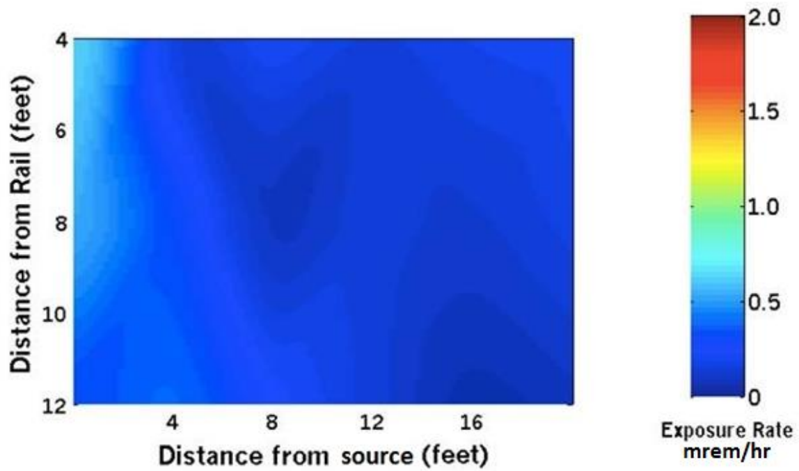
Figure 11: Plot of exposure rates 3 feet above the surface of the tie.
