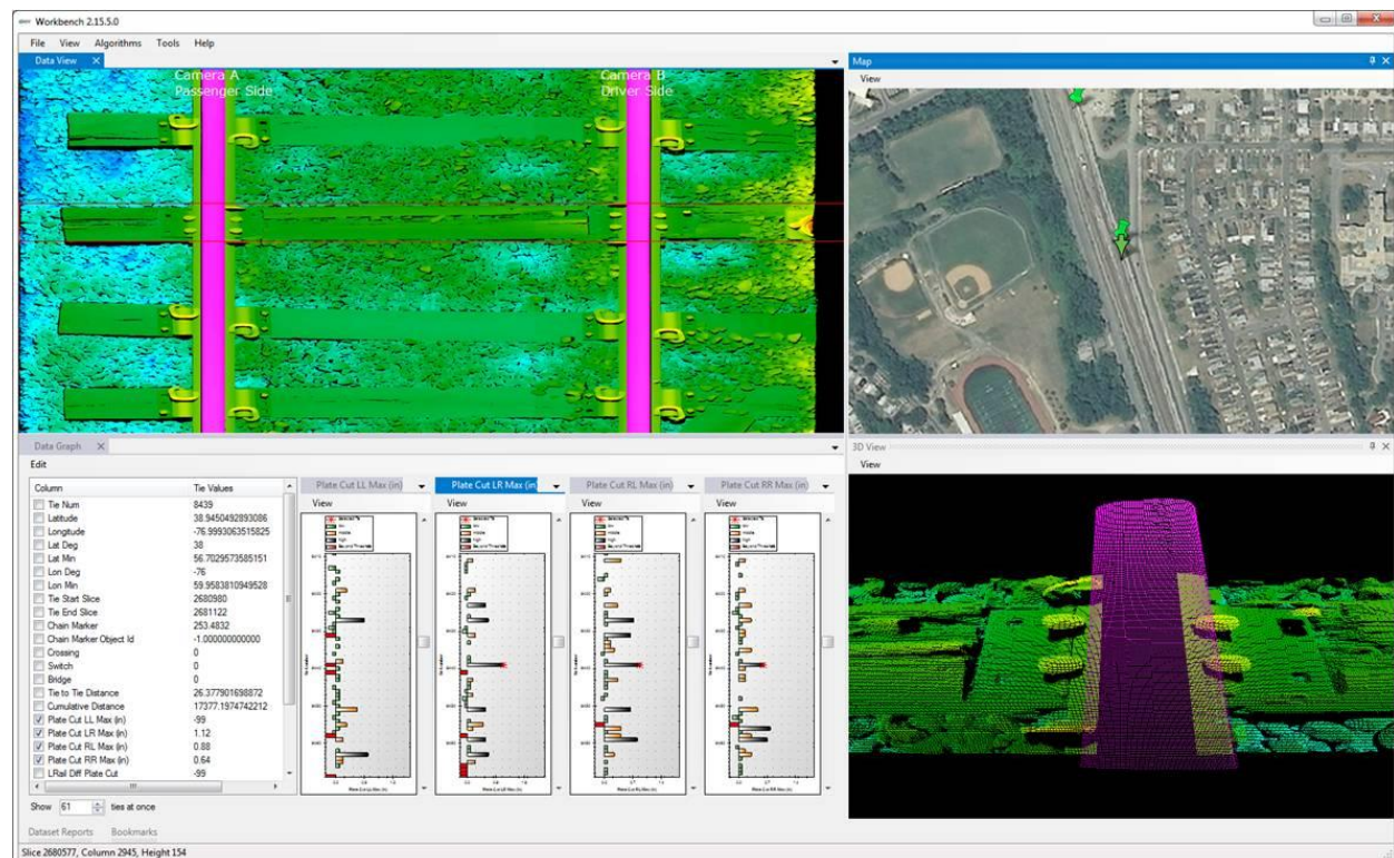
Figure 1: Aurora tie grading and planning system. Top Left is a 2-dimensional overview of track bed. Top Right is a map overview of tie locations based on GPS and Milepost coordinates. Bottom Left are individual measurements for a series of ties. Bottom Right is a 3-dimensional view of track bed.
