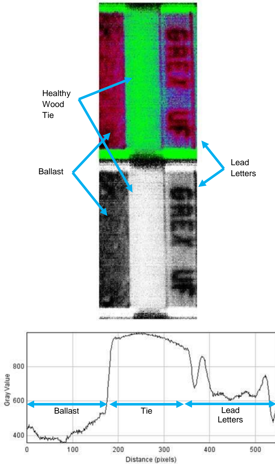
Figure 6: Various images of a healthy wood tie. Top: Colored Image. Center: Grayscale Image. Bottom: Average Density Profile in the longitudinal direction.
